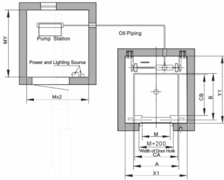
Ichnography of Hoistway and Machine Room
