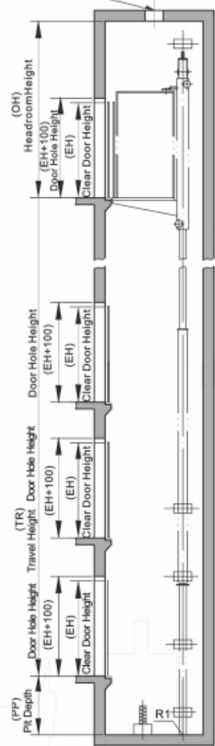
Hoistway Vertical View
