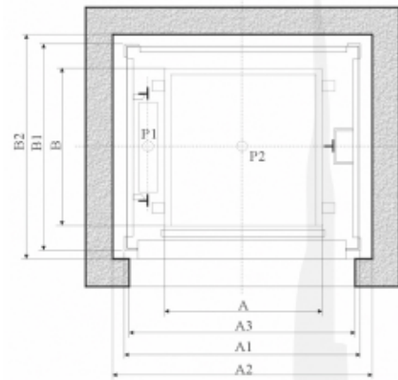
Plan of Hoistway and Machine room Door opposite opening
