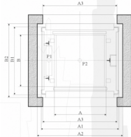
Plan of Hoistway and Machine room Door opposite opening
