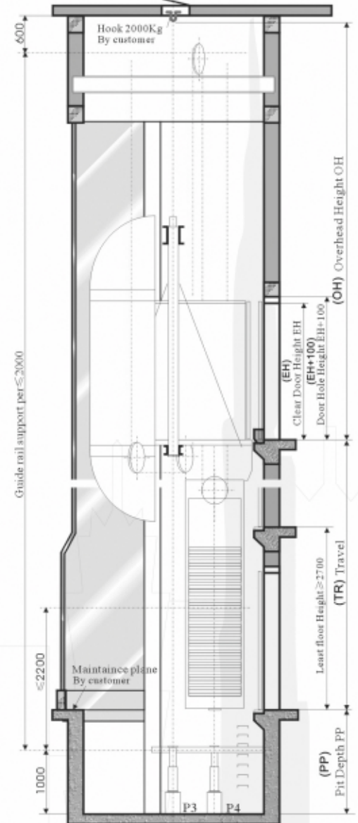
Hoistway Cutaway View
