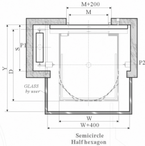
Plan of Hoistway and Machine room
